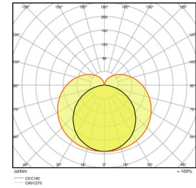
LINEAR LED 1200 20 W 3000 K POWER
